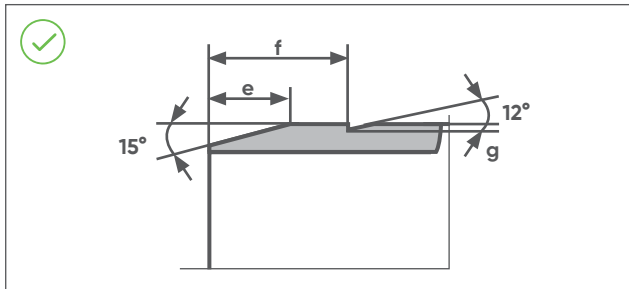
Illustration 7.24 Snap joint
