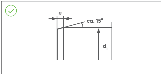
Illustration 7.23 Plug-in joint
